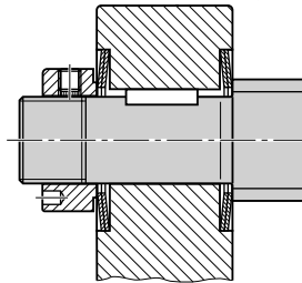
Mounting with cup spring
