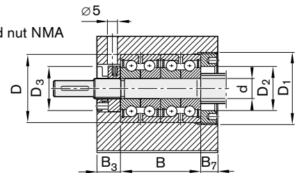
LGN-C-... with slotted nut NMA
